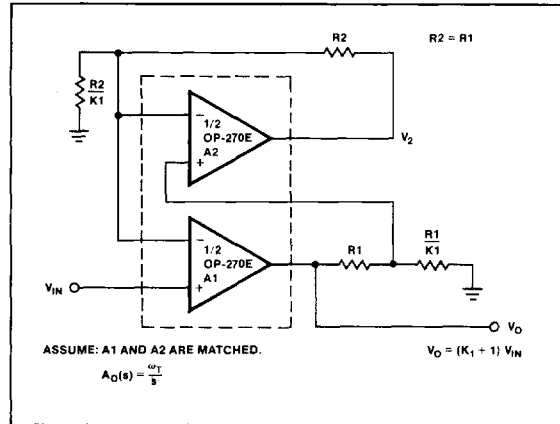
FIGURE 10: Low Phase Error Amplifier
