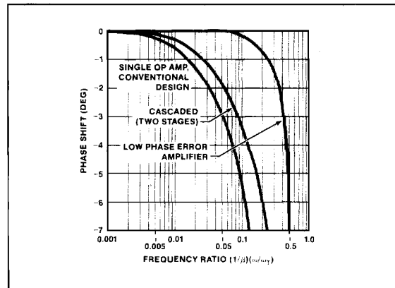
FIGURE 11: Phase Error Comparison
