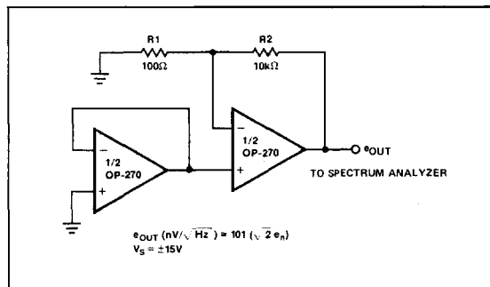
FIGURE 6: Noise Voltage Density Test Circuit
