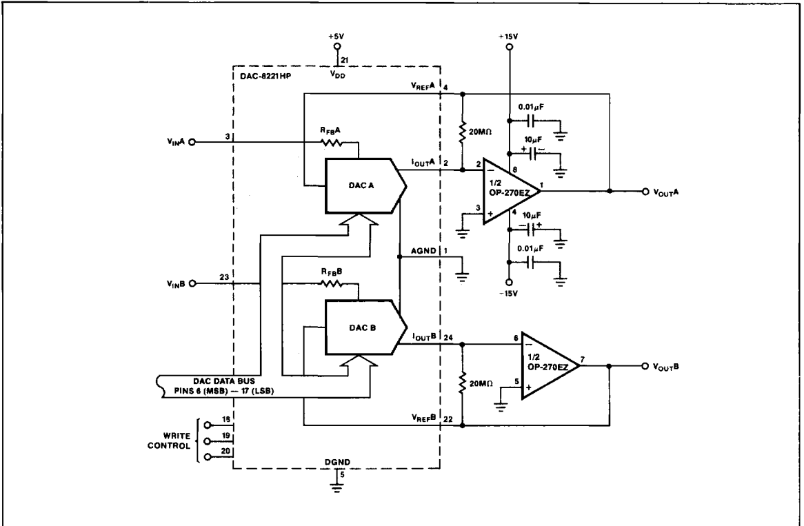
FIGURE 15: Dual Programmable Gain Amplifier
