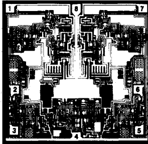
DIE SIZE 0.094 × 0.092 inch, 8,648 sq. mils (2.39 × 2.34 mm, 5.60 sq. mm)
