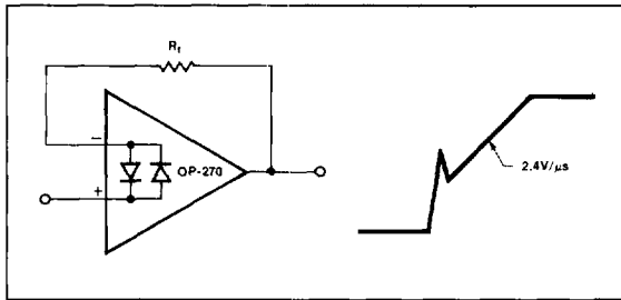
FIGURE 9: Pulsed Operation
